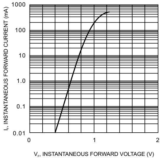
FIG.1- FORWARD CHARACTERISTICS
