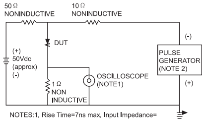
FIG.5- REVERSE RECOVER TIME CHARACTERISTIC AND TEST CIRCUIT DIAGRAM
