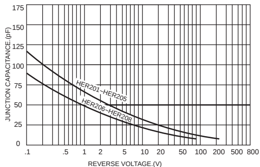
FIG.6-TYPICAL JUNCTION CHARACTERISTICS
