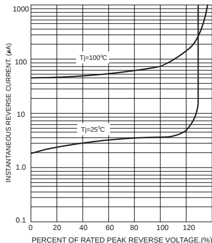
FIG.3-TYPICAL REVERSE CHARACTERISTICS
