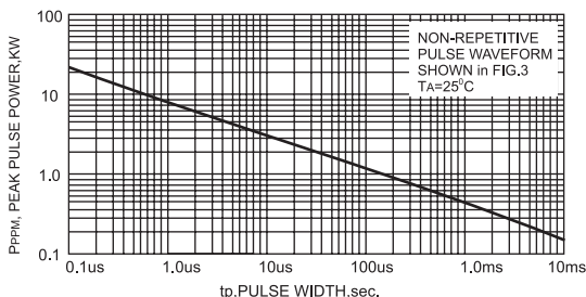
FIG.1- PEAK PULSE POWER RATING CURVE
