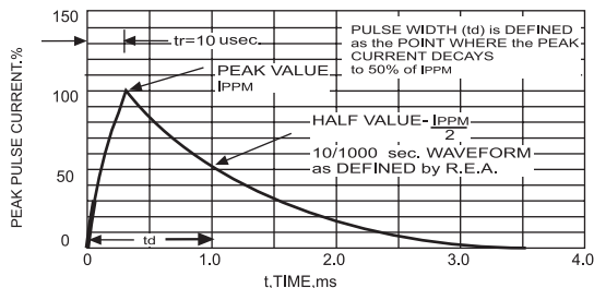
FIG.3- PULSE WAVEFORM
