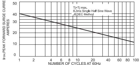
FIG.5-MAXIMUM NON-REPETITIVE FORWARD SURGE CURRENT UNIDIRECTIONAL ONLY
