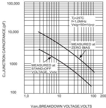
FIG.7-TYPICAL JUNCTION CAPACITANCE UNIDIRECTIONAL
