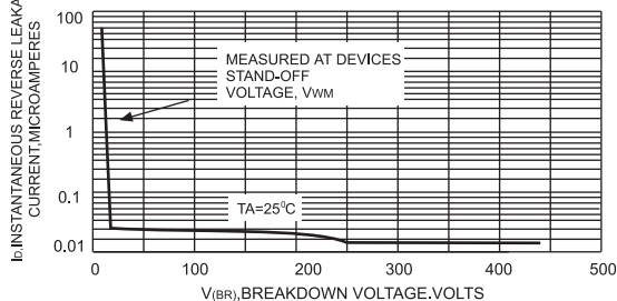
FIG.6-TYPICAL REVERSE LEAKAGE CHARACTERISTICS
