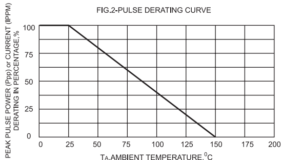
FIG.2-PULSE DERATING CURVE
