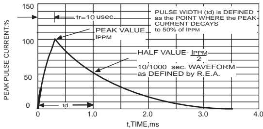
FIG.3- PULSE WAVEFORM
