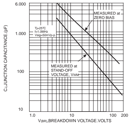
FIG.7-TYPICAL JUNCTION CAPACITANCE UNIDIRECTIONAL
