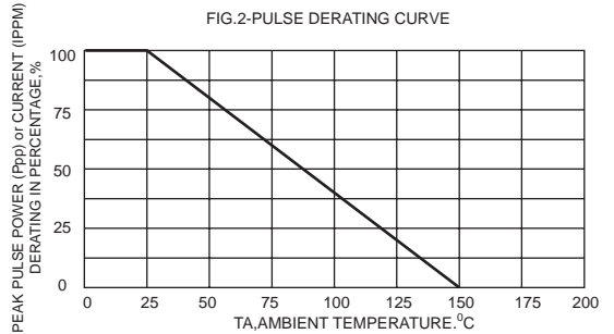
FIG.2-PULSE DERATING CURVE
