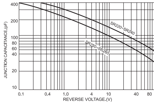
FIG.4-TYPICAL JUNCTION CAPACITANCE
